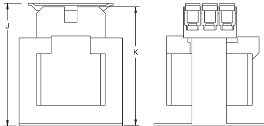
Transformer with Fuse Holder and Covers
