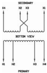
Primary — 480V
