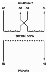
Primary — 480V
