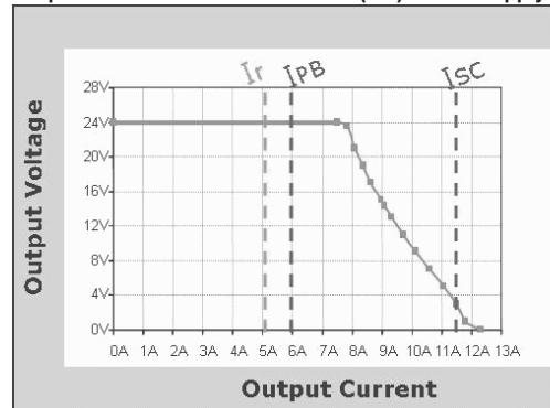
Output Characteristic for XLS120E (5 A) Power Supply
